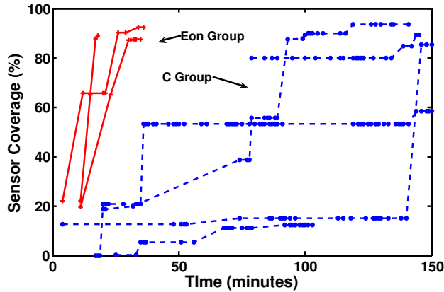
Figure 8. Percent sensor coverage (best so far) is shown comparing C and Eon programmers. By separating adaptation policy from execution, Eon users were able to build high-performing adaptive sensor applications significantly faster than those using C.
