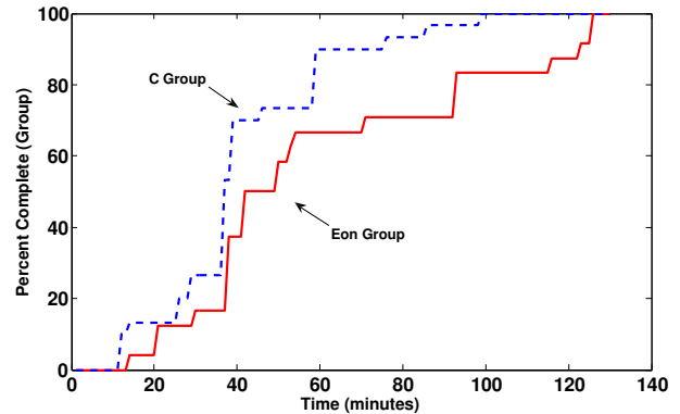
Figure 7. This figure compares experienced C programmers with first-time Eon users programming a simple sensor application. Aggregate group progress is shown over time. Despite language differences, both groups’ progression is surprisingly similar. Small differences are likely due to the overhead of learning a new language.
