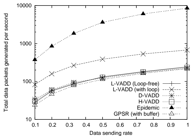
Fig. 12. The number of packets generated
