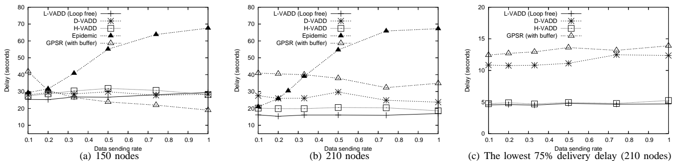
Fig. 11. Data delivery delay as a function of the data sending rate
