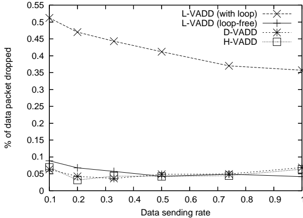
Fig. 10. Percent of data packets dropped due to routing loops or MAC layer packet collisions (150 nodes)
