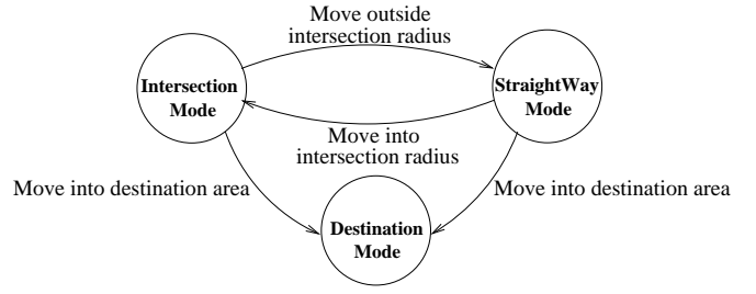
Fig. 2. The transition modes in VADD
