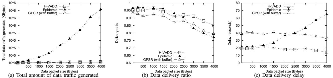
Fig. 13. Impact of data packet size
