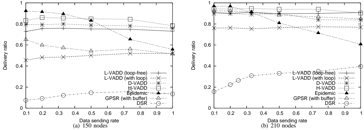
Fig. 9. Data delivery ratio as a function of the data sending rate
