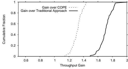
(a) CDF of throughputs for Alice-Bob topology
